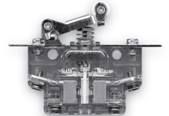
S800 aL Version with roller lever, mounting brackets, silver contacts, M3 screws with saddle clamp and blowouts
