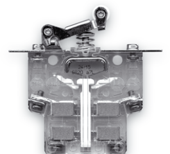
S820 a7 Version with roller lever, mounting brackets, silver contacts and M3 screws with saddle clamp
